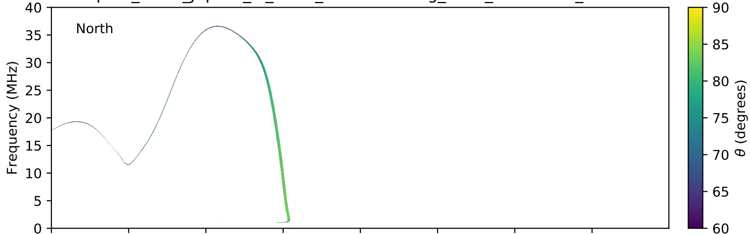
expres_earth_jupiter_io_isaac_lossc-wid1deg_3kev_20160917_v01.cdf
