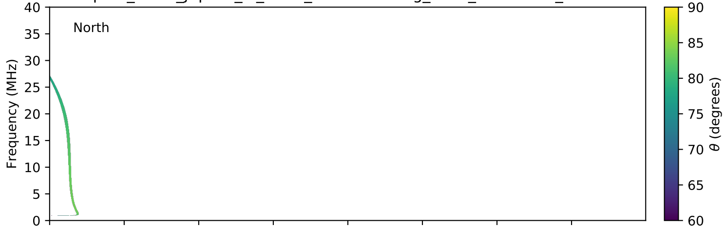
expres_earth_jupiter_io_isaac_lossc-wid1deg_3kev_20160912_v01.cdf
