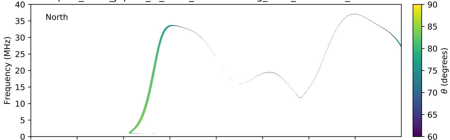
expres_earth_jupiter_io_isaac_lossc-wid1deg_3kev_20160911_v01.cdf
