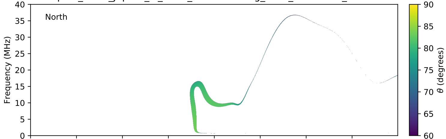
expres_earth_jupiter_io_isaac_lossc-wid1deg_3kev_20160909_v01.cdf
