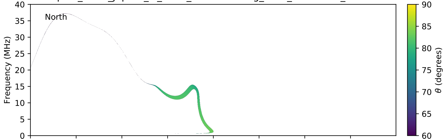
expres_earth_jupiter_io_isaac_lossc-wid1deg_3kev_20160908_v01.cdf
