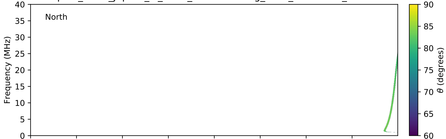
expres_earth_jupiter_io_isaac_lossc-wid1deg_3kev_20160905_v01.cdf
