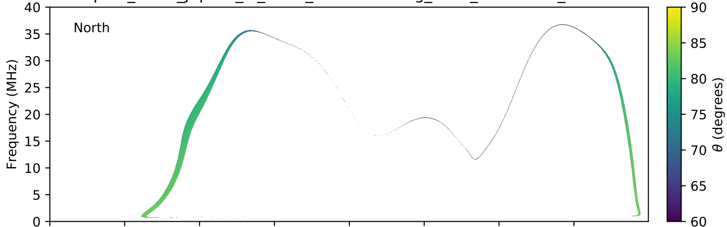
expres_earth_jupiter_io_isaac_lossc-wid1deg_3kev_20160904_v01.cdf
