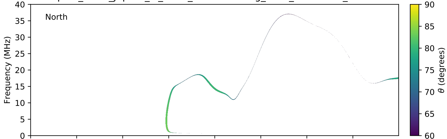
expres_earth_jupiter_io_isaac_lossc-wid1deg_3kev_20160902_v01.cdf
