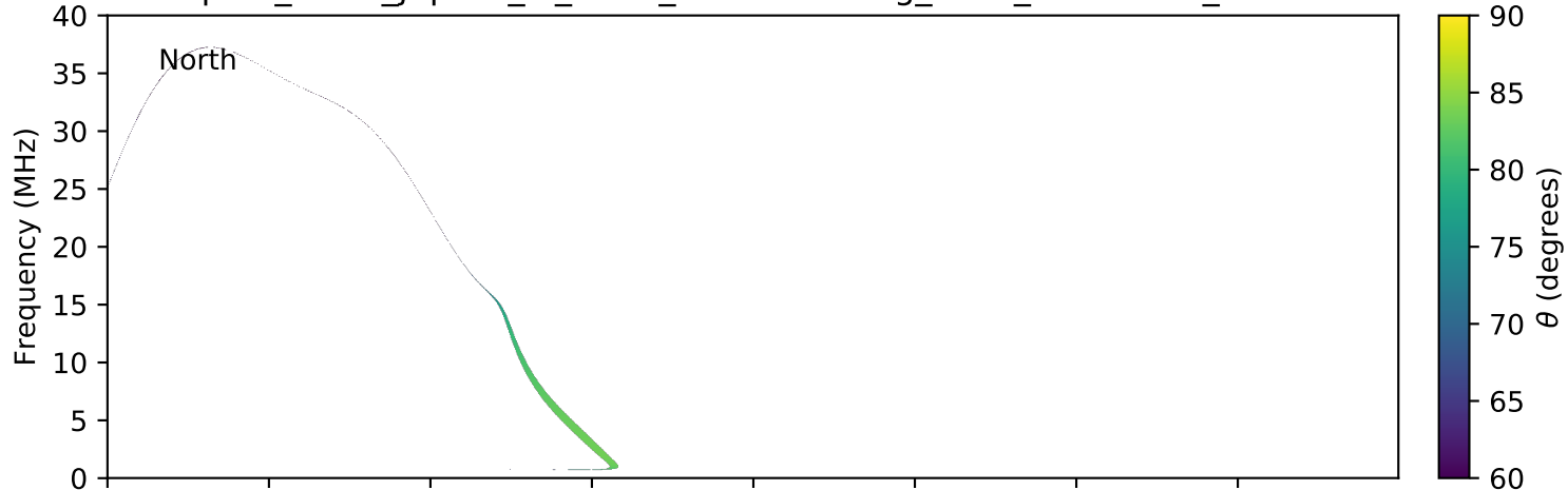
expres_earth_jupiter_io_isaac_lossc-wid1deg_3kev_20160901_v01.cdf
