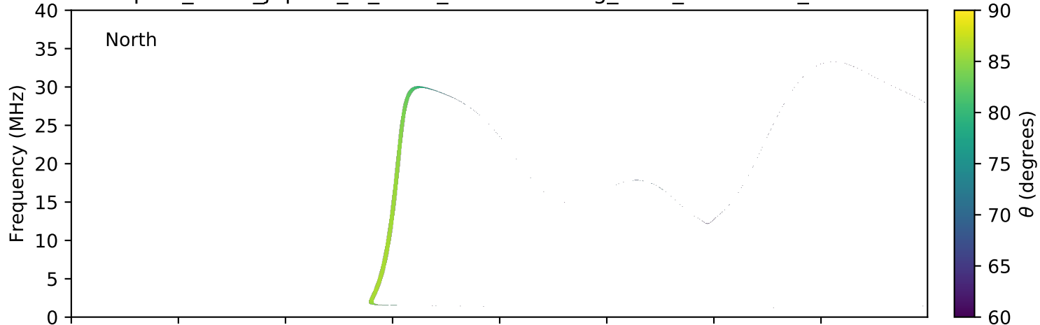
expres_earth_jupiter_io_isaac_lossc-wid1deg_1kev_20160918_v01.cdf
