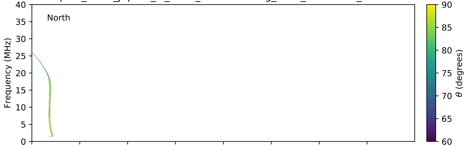
expres_earth_jupiter_io_isaac_lossc-wid1deg_1kev_20160912_v01.cdf
