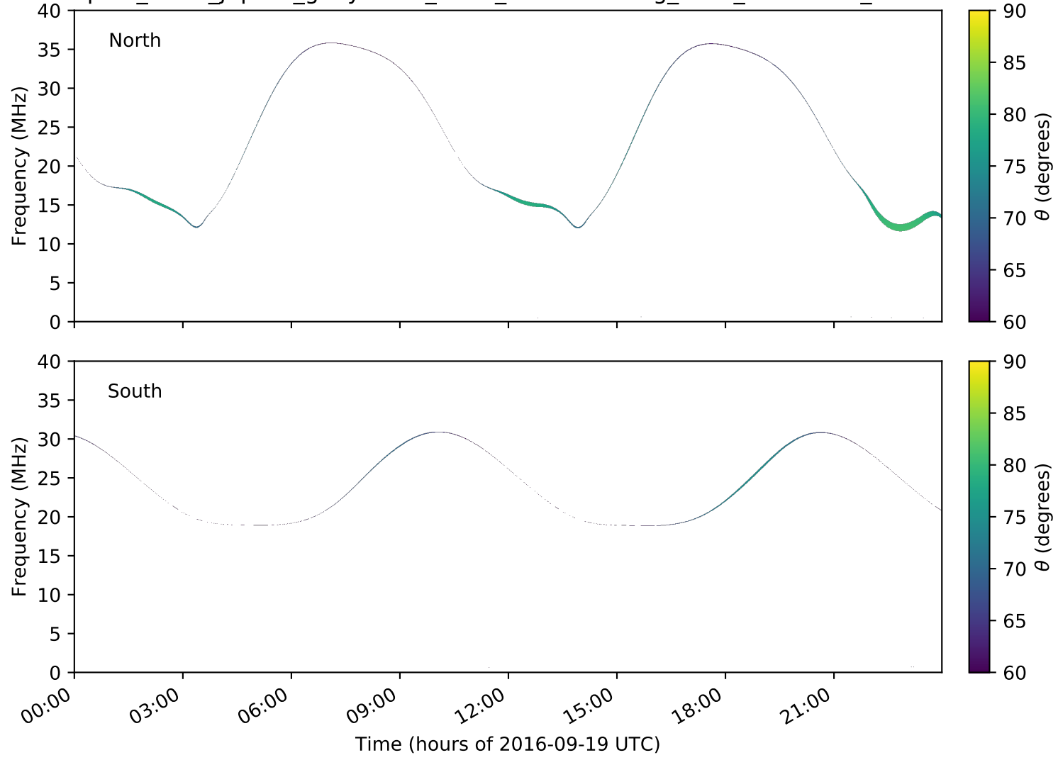
expres_earth_jupiter_ganymede_isaac_lossc-wid1deg_3kev_20160919_v01.cdf
