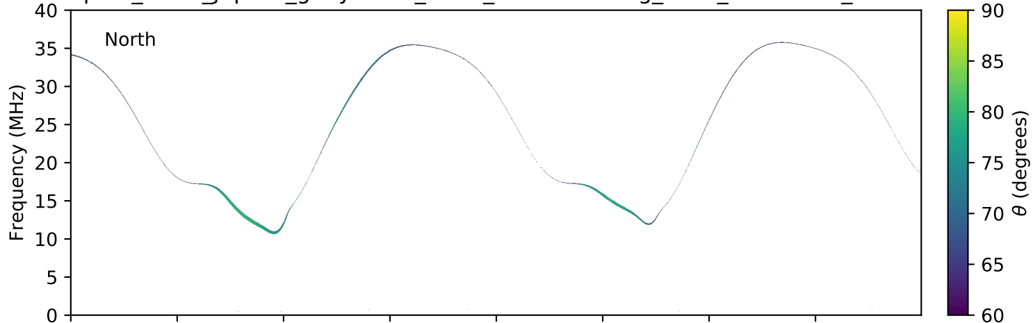
expres_earth_jupiter_ganymede_isaac_lossc-wid1deg_3kev_20160911_v01.cdf
