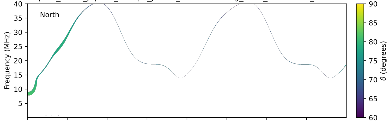
expres_earth_jupiter_europa_jrm33_lossc-wid1deg_3kev_20160917_v11.cdf
