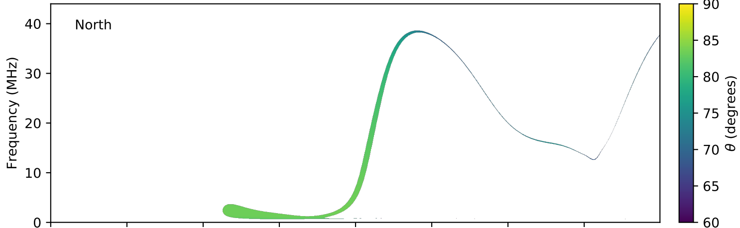
expres_earth_jupiter_europa_jrm09_lossc-wid1deg_3kev_20160929_v01.cdf
