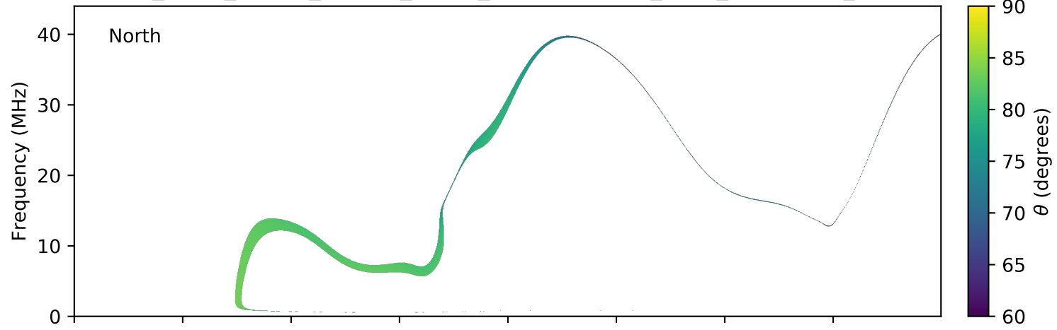
expres_earth_jupiter_europa_jrm09_lossc-wid1deg_3kev_20160922_v01.cdf
