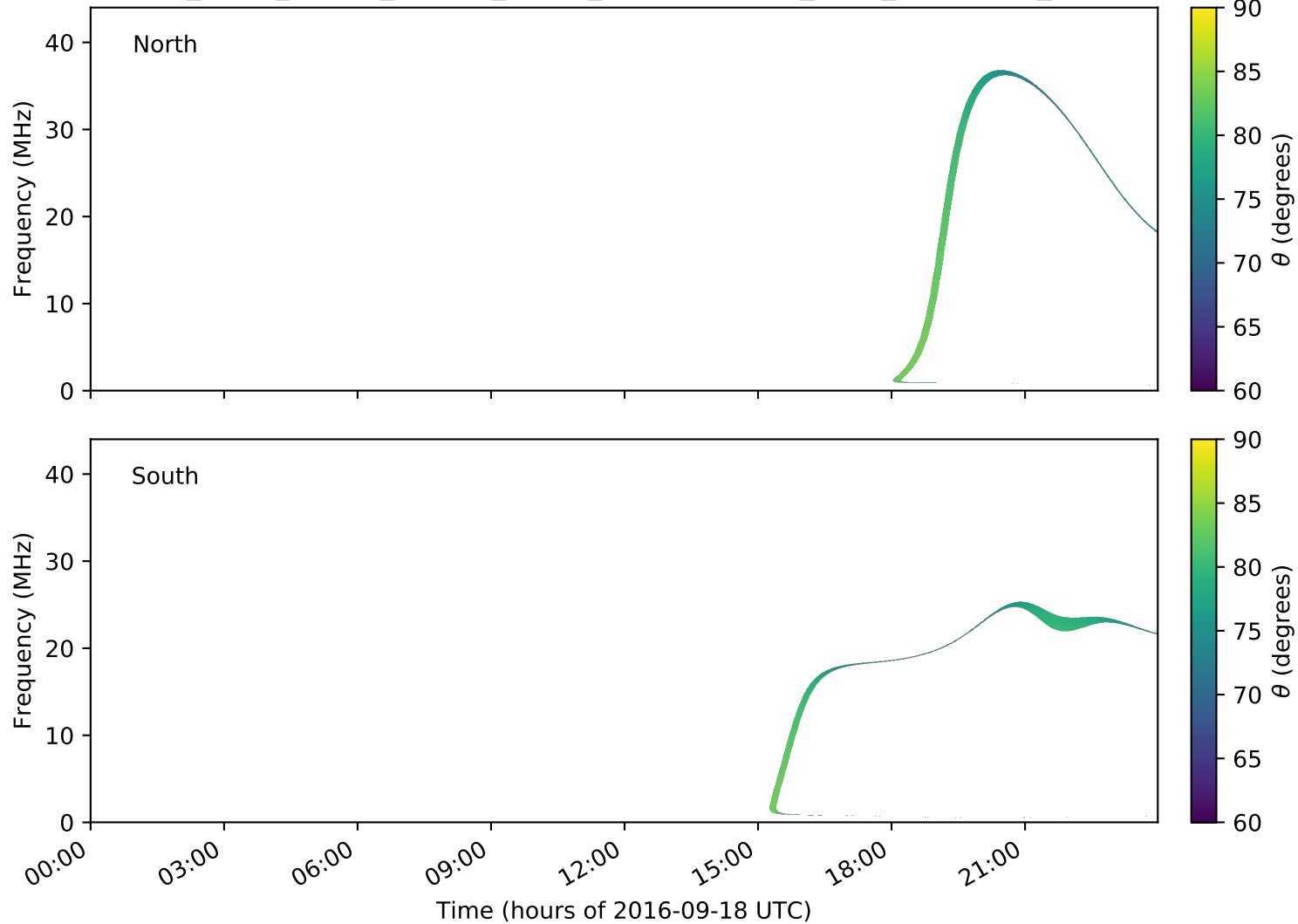
expres_earth_jupiter_europa_jrm09_lossc-wid1deg_3kev_20160918_v01.cdf
