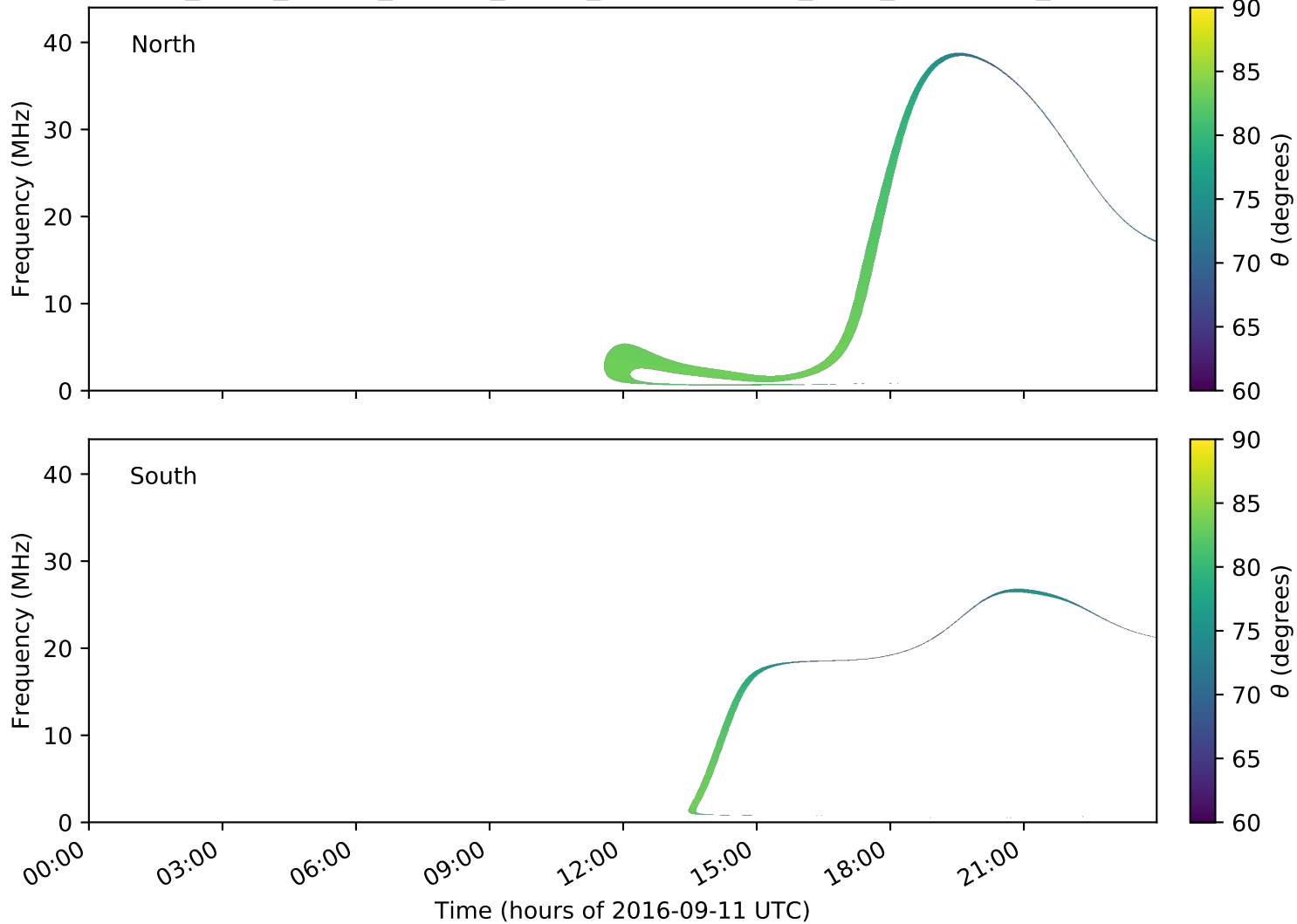
expres_earth_jupiter_europa_jrm09_lossc-wid1deg_3kev_20160911_v01.cdf
