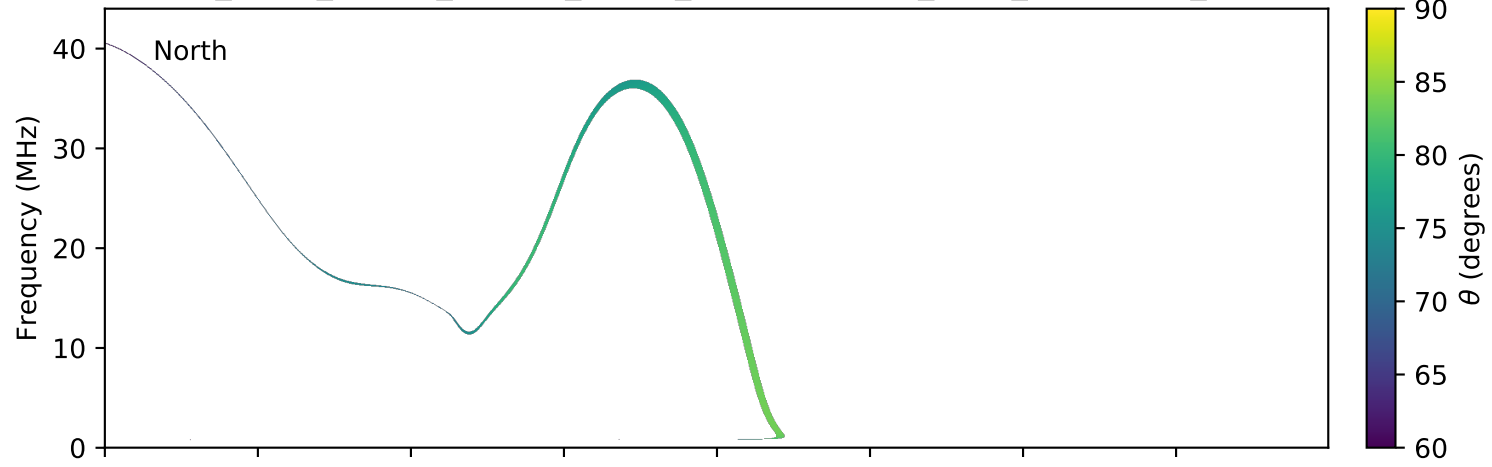
expres_earth_jupiter_europa_jrm09_lossc-wid1deg_3kev_20160909_v01.cdf
