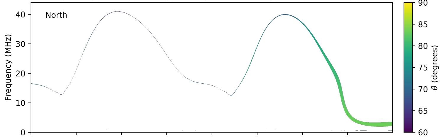
expres_earth_jupiter_europa_jrm09_lossc-wid1deg_3kev_20160905_v01.cdf
