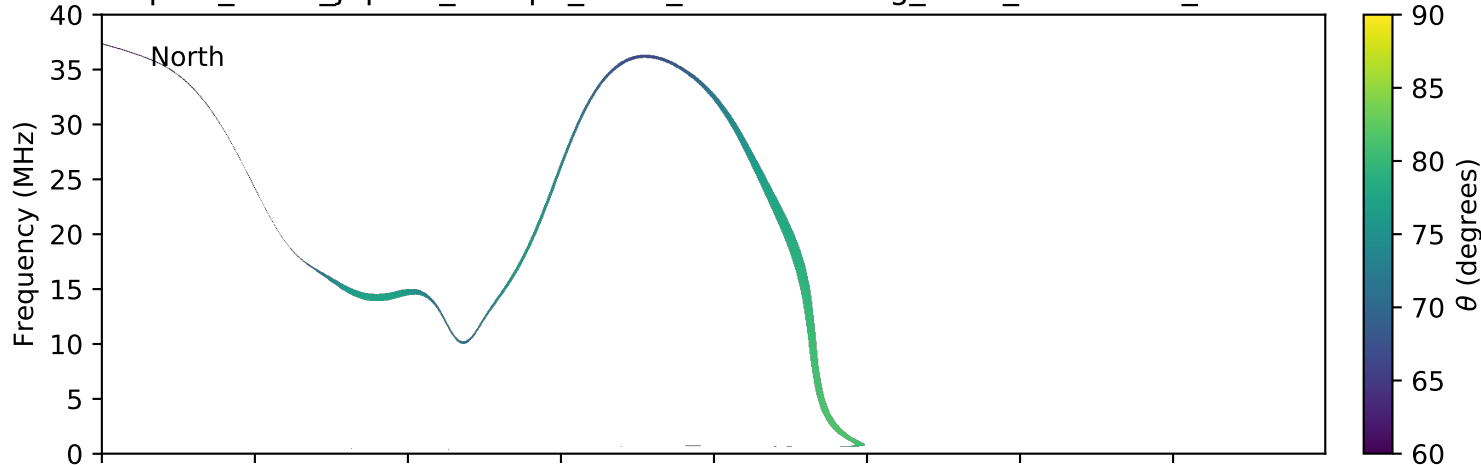
expres_earth_jupiter_europa_isaac_lossc-wid1deg_5kev_20160916_v01.cdf
