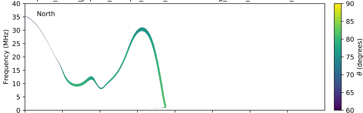
expres_earth_jupiter_europa_isaac_lossc-wid1deg_5kev_20160902_v01.cdf
