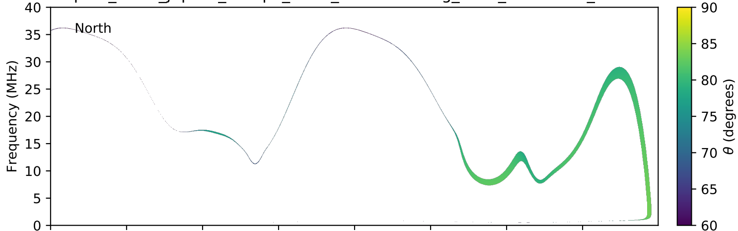
expres_earth_jupiter_europa_isaac_lossc-wid1deg_3kev_20160930_v01.cdf
