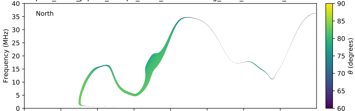
expres_earth_jupiter_europa_isaac_lossc-wid1deg_3kev_20160922_v01.cdf
