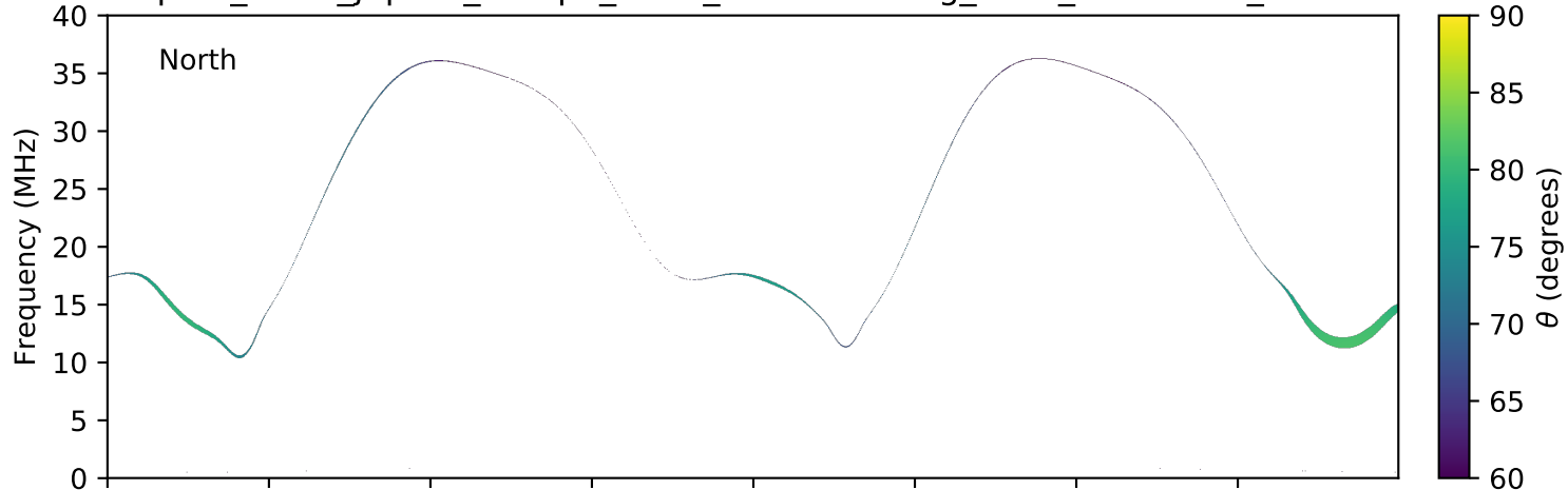
expres_earth_jupiter_europa_isaac_lossc-wid1deg_3kev_20160919_v01.cdf
