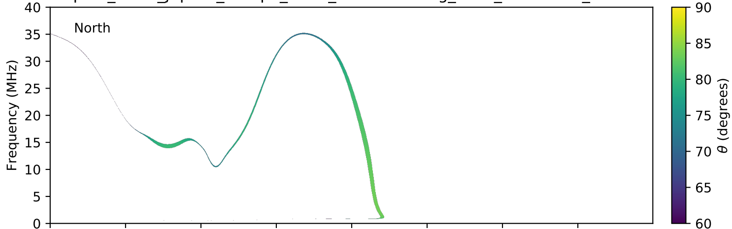
expres_earth_jupiter_europa_isaac_lossc-wid1deg_3kev_20160909_v01.cdf
