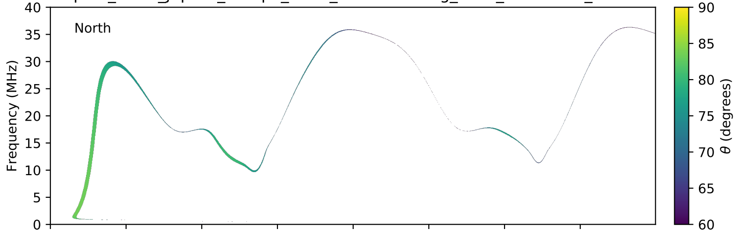
expres_earth_jupiter_europa_isaac_lossc-wid1deg_3kev_20160908_v01.cdf
