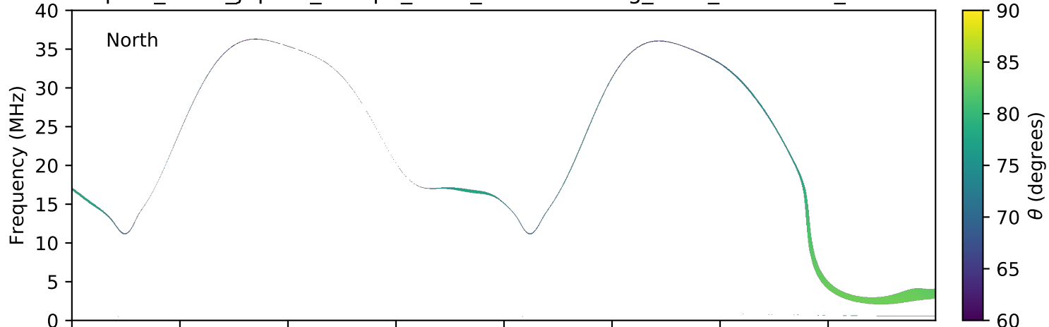
expres_earth_jupiter_europa_isaac_lossc-wid1deg_3kev_20160905_v01.cdf
