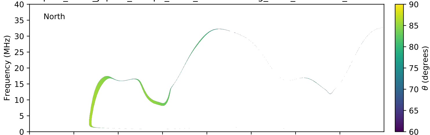
expres_earth_jupiter_europa_isaac_lossc-wid1deg_1kev_20160922_v01.cdf
