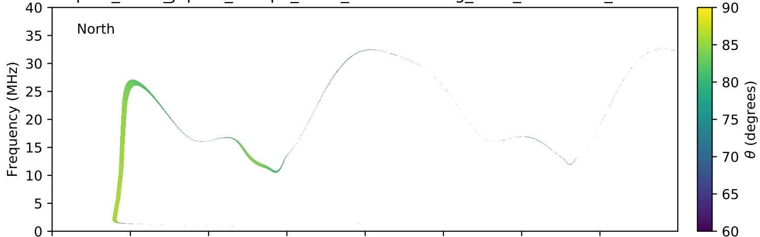
expres_earth_jupiter_europa_isaac_lossc-wid1deg_1kev_20160915_v01.cdf
