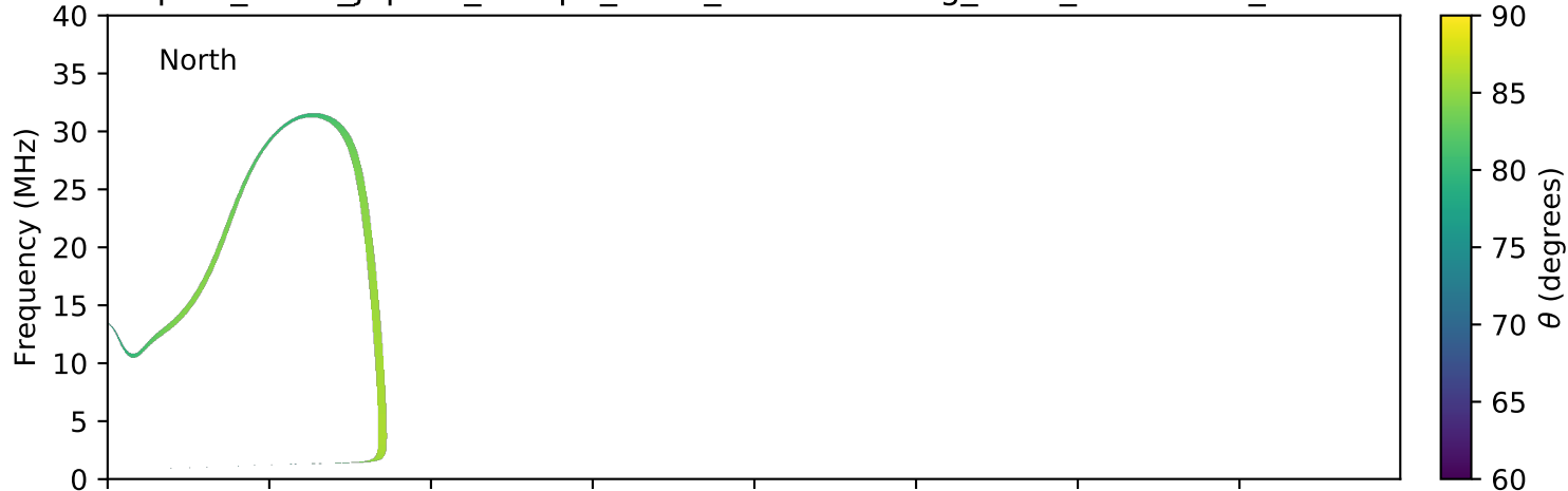
expres_earth_jupiter_europa_isaac_lossc-wid1deg_1kev_20160913_v01.cdf
