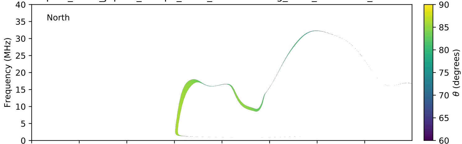
expres_earth_jupiter_europa_isaac_lossc-wid1deg_1kev_20160904_v01.cdf
