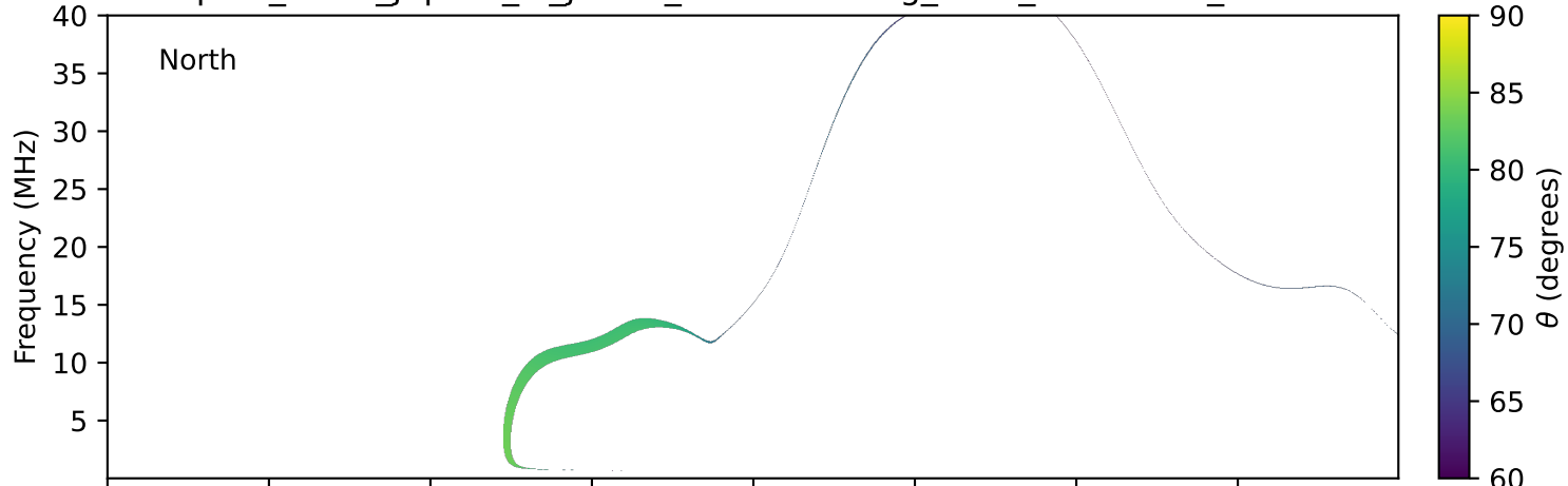
expres_earth_jupiter_io_jrm33_lossc-wid1deg_3kev_20160625_v11.cdf
