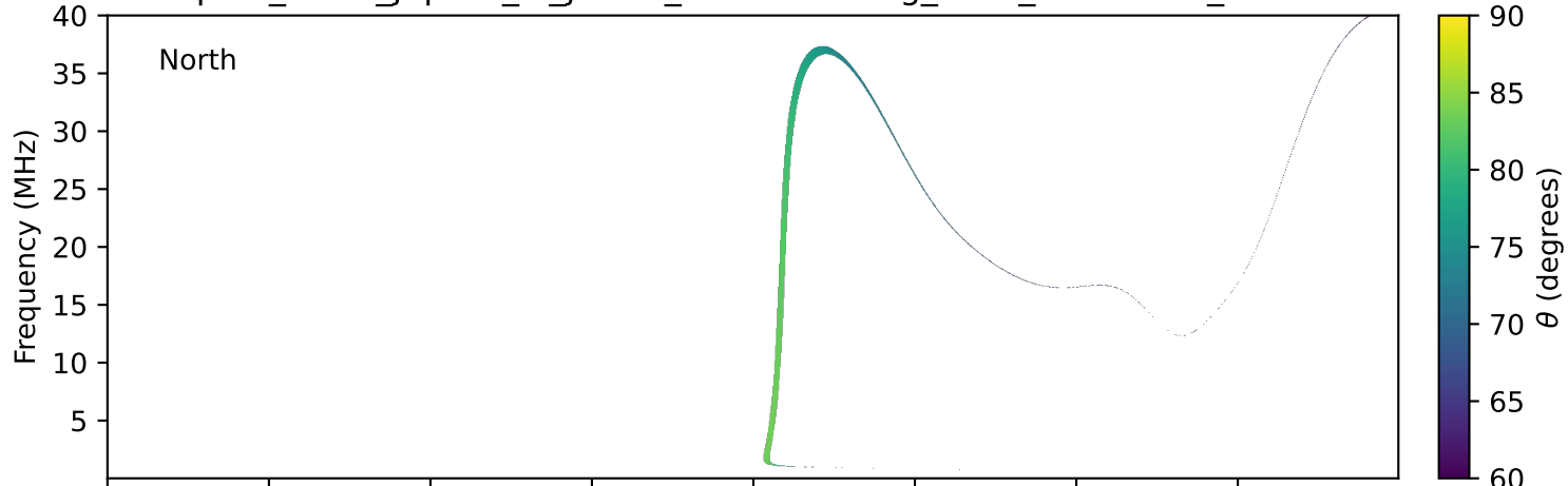
expres_earth_jupiter_io_jrm33_lossc-wid1deg_3kev_20160616_v11.cdf
