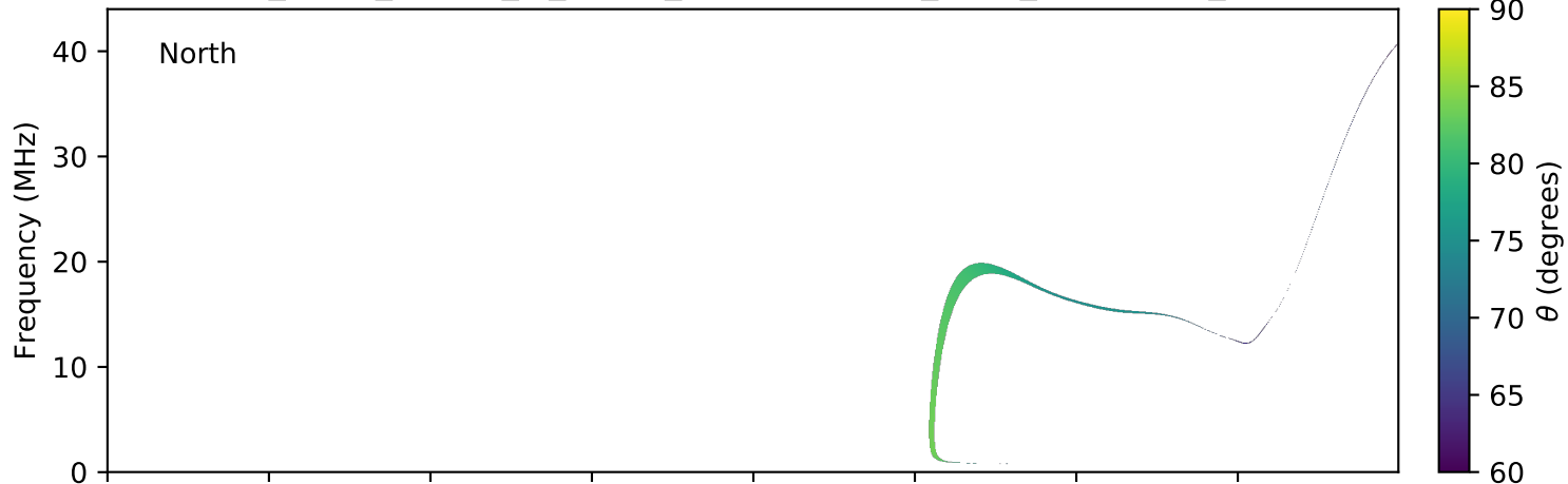
expres_earth_jupiter_io_jrm09_lossc-wid1deg_3kev_20160630_v01.cdf
