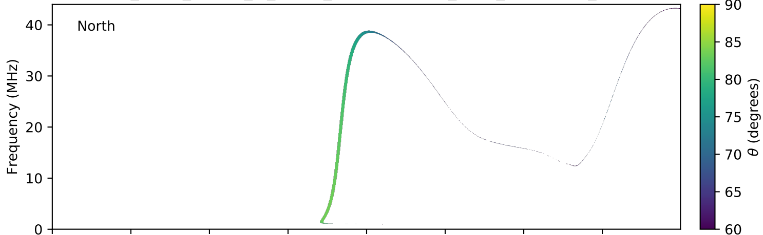
expres_earth_jupiter_io_jrm09_lossc-wid1deg_3kev_20160609_v01.cdf
