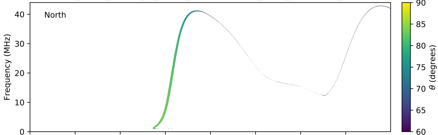
expres_earth_jupiter_io_jrm09_lossc-wid1deg_3kev_20160602_v01.cdf
