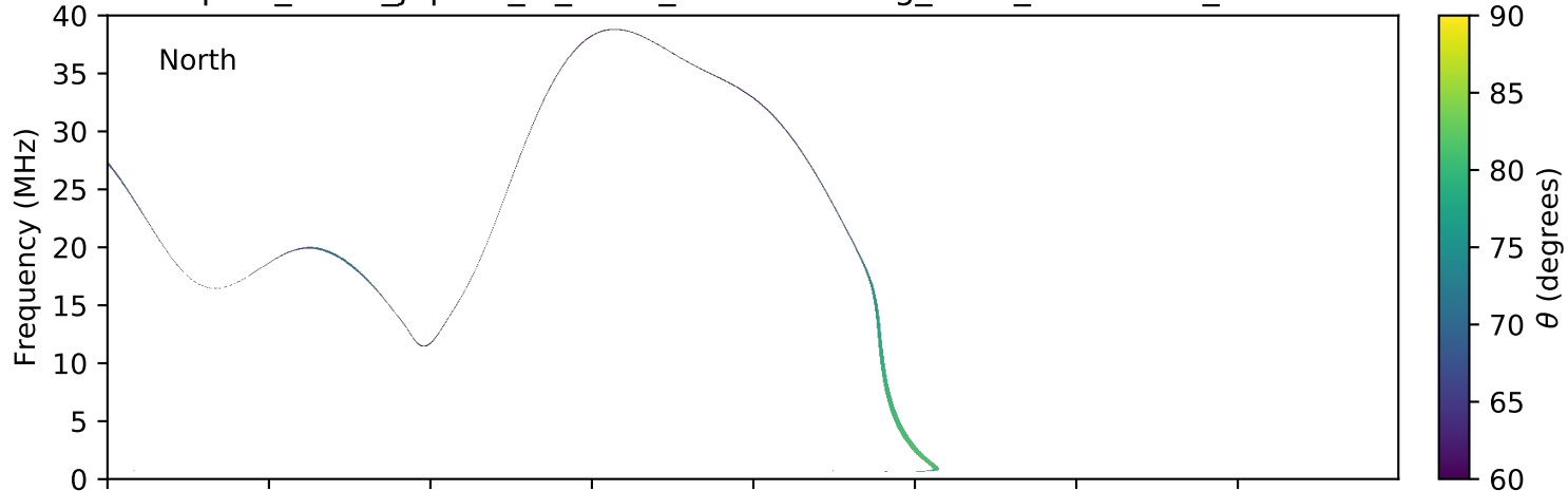
expres_earth_jupiter_io_isaac_lossc-wid1deg_5kev_20160629_v01.cdf
