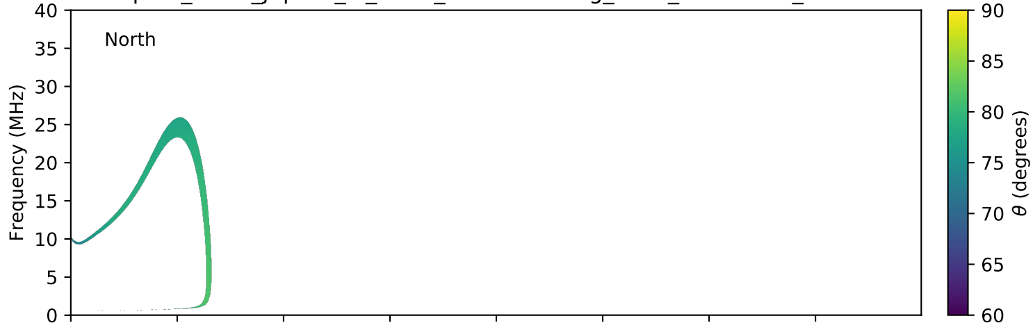
expres_earth_jupiter_io_isaac_lossc-wid1deg_5kev_20160626_v01.cdf
