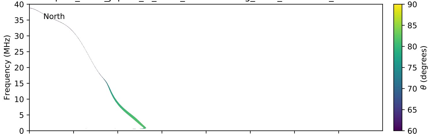
expres_earth_jupiter_io_isaac_lossc-wid1deg_5kev_20160624_v01.cdf
