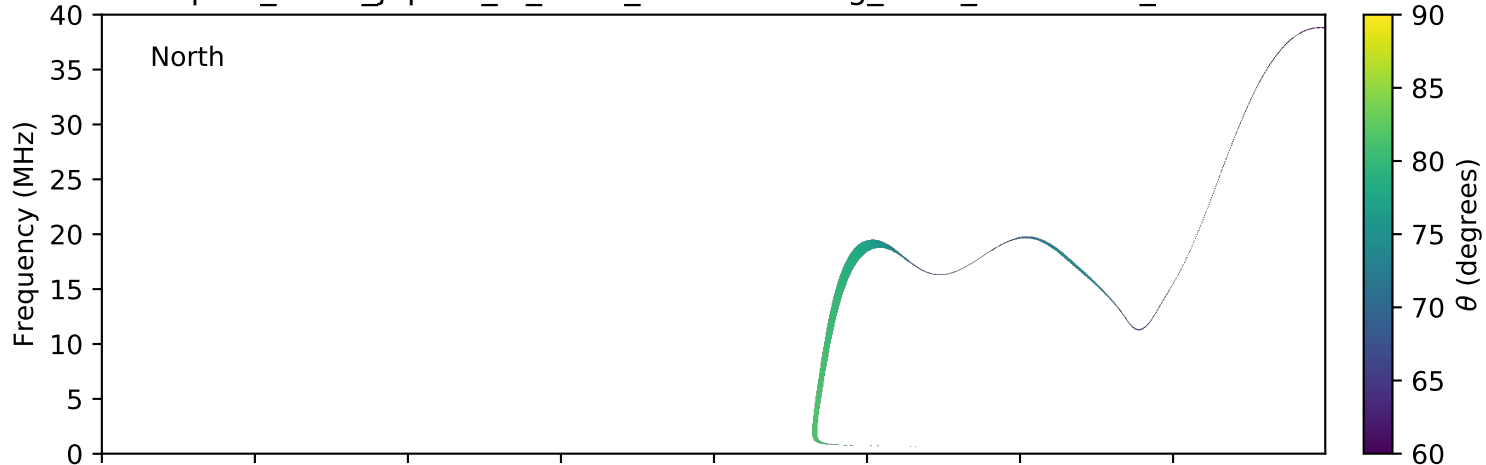
expres_earth_jupiter_io_isaac_lossc-wid1deg_5kev_20160623_v01.cdf
