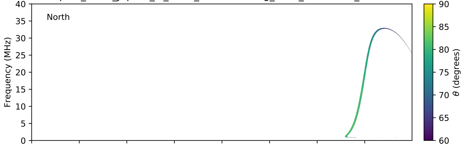
expres_earth_jupiter_io_isaac_lossc-wid1deg_5kev_20160621_v01.cdf
