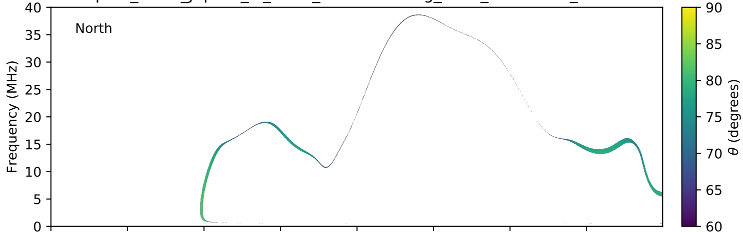
expres_earth_jupiter_io_isaac_lossc-wid1deg_5kev_20160618_v01.cdf
