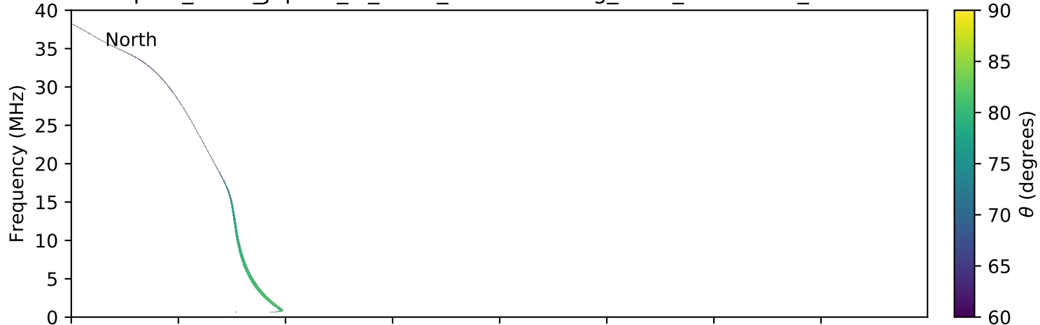
expres_earth_jupiter_io_isaac_lossc-wid1deg_5kev_20160617_v01.cdf
