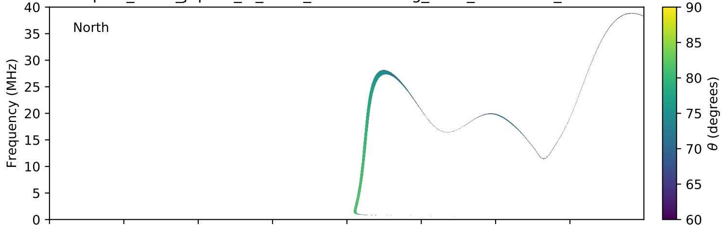
expres_earth_jupiter_io_isaac_lossc-wid1deg_5kev_20160616_v01.cdf
