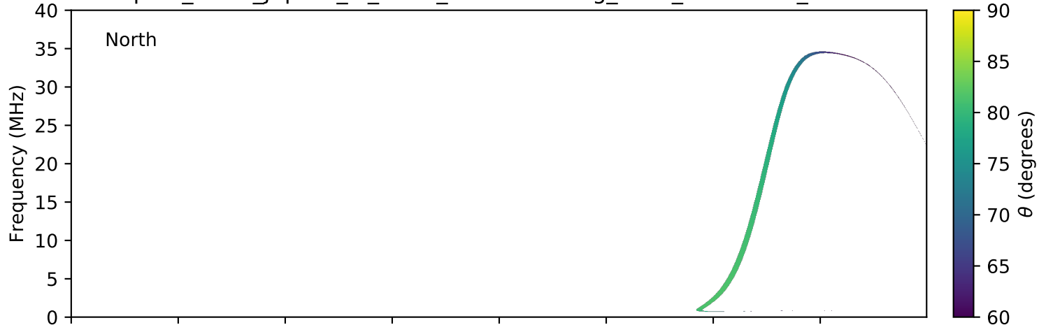
expres_earth_jupiter_io_isaac_lossc-wid1deg_5kev_20160614_v01.cdf
