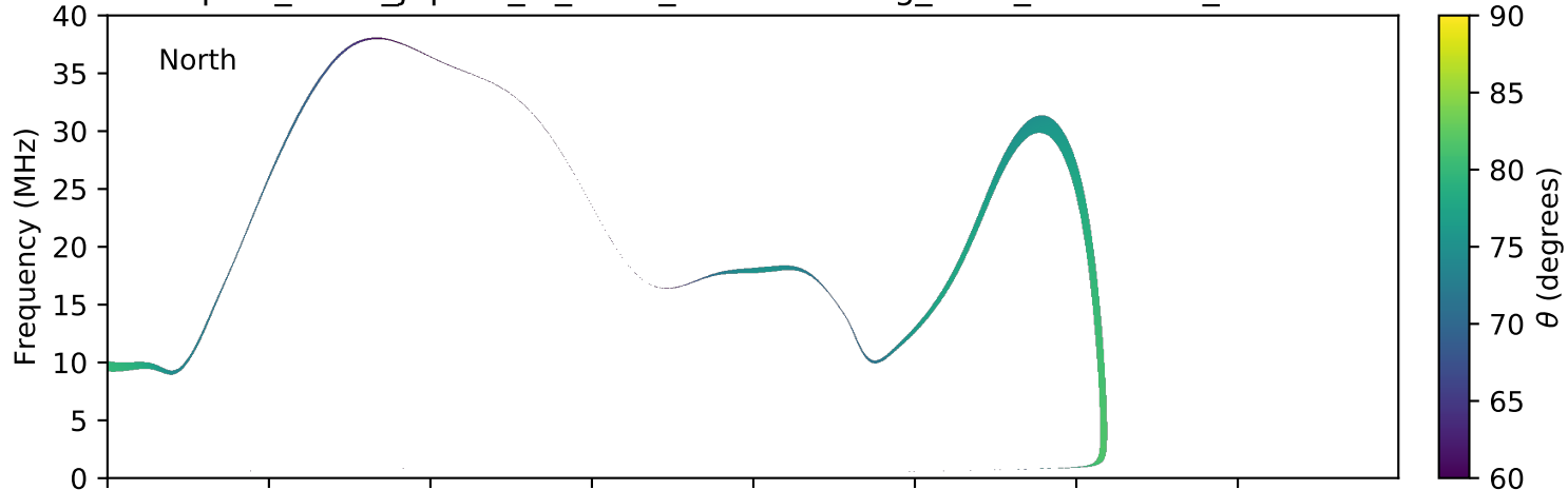
expres_earth_jupiter_io_isaac_lossc-wid1deg_5kev_20160613_v01.cdf
