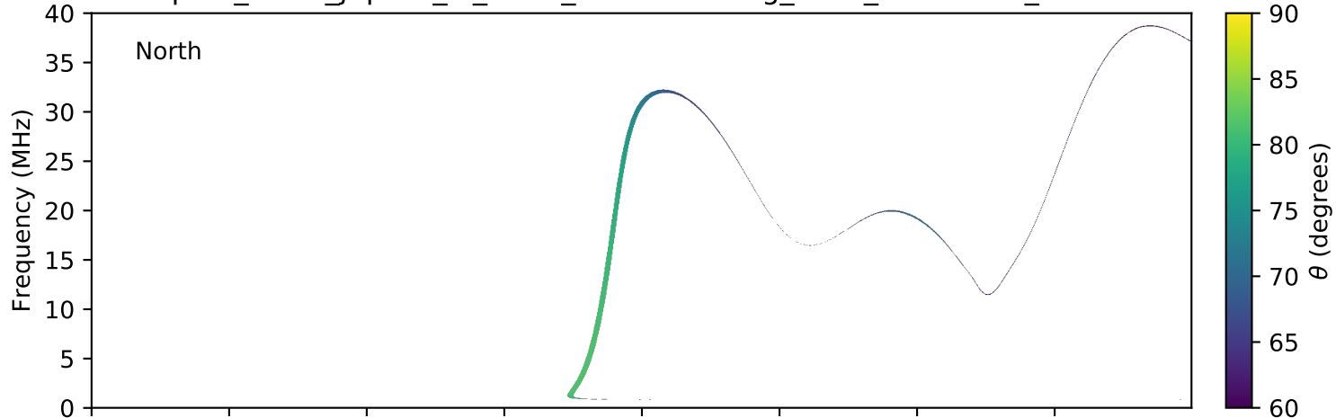
expres_earth_jupiter_io_isaac_lossc-wid1deg_5kev_20160609_v01.cdf
