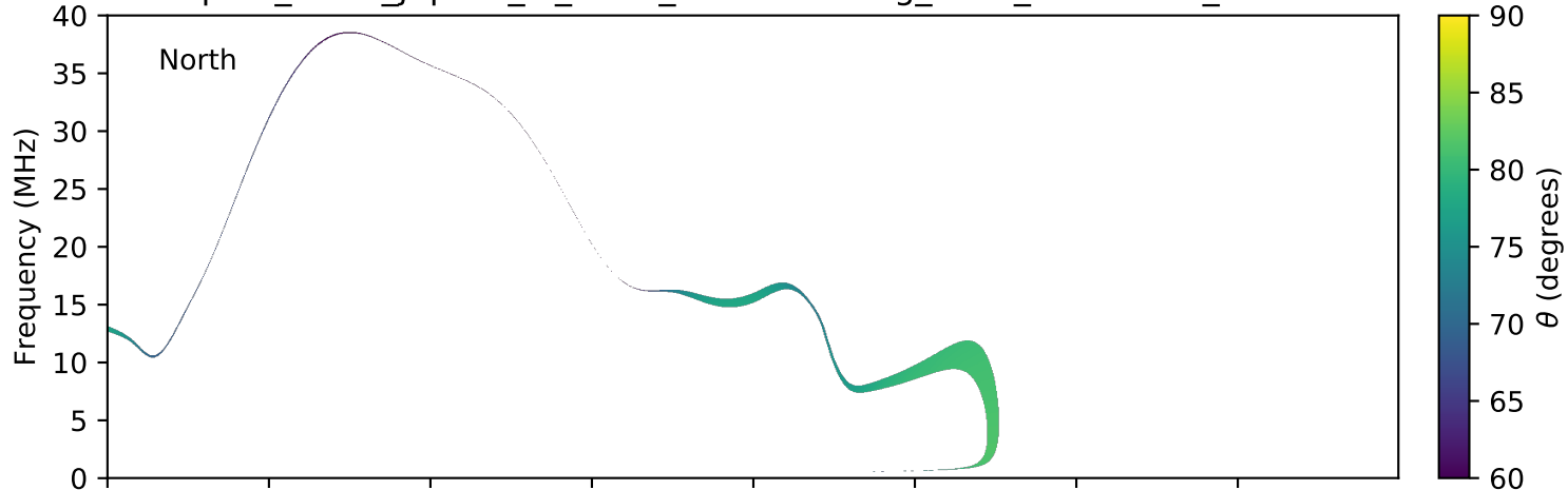
expres_earth_jupiter_io_isaac_lossc-wid1deg_5kev_20160606_v01.cdf
