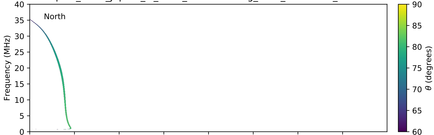
expres_earth_jupiter_io_isaac_lossc-wid1deg_5kev_20160603_v01.cdf
